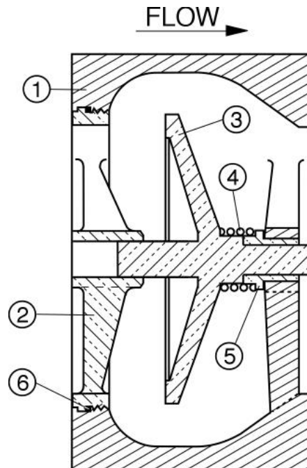
FIGURE 4. WAFER STYLE CHECK VALVE
