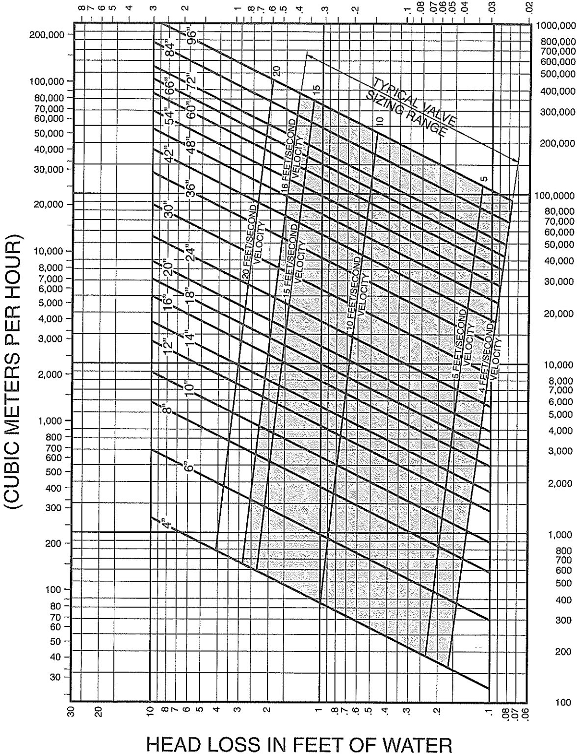
HEAD LOSS CHART FOR CLASS 150B AND 250B BUTTERFLY VALVES
