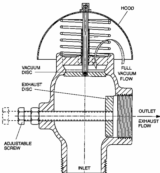
Dual-Port Throttling Device
