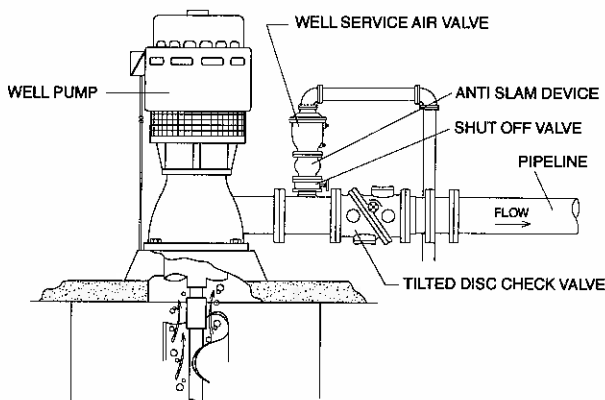
Vertical Turbine Pump
